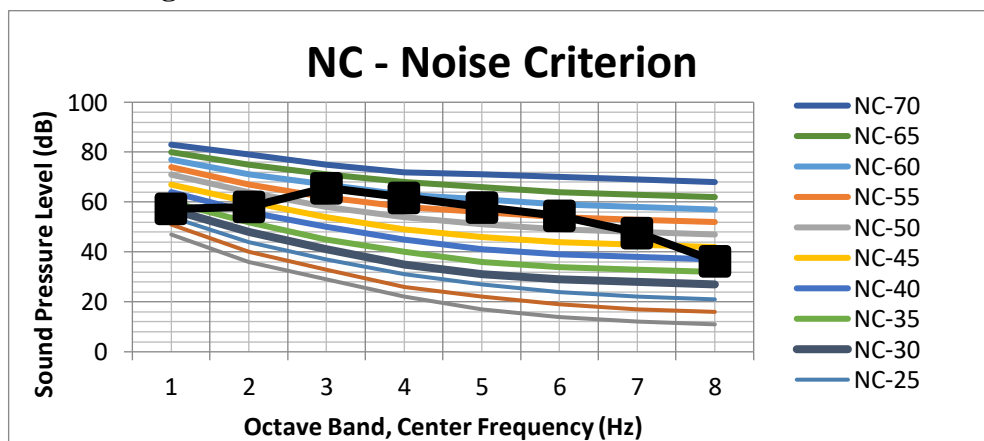
Gambar 4 grafik NC Background Noise
