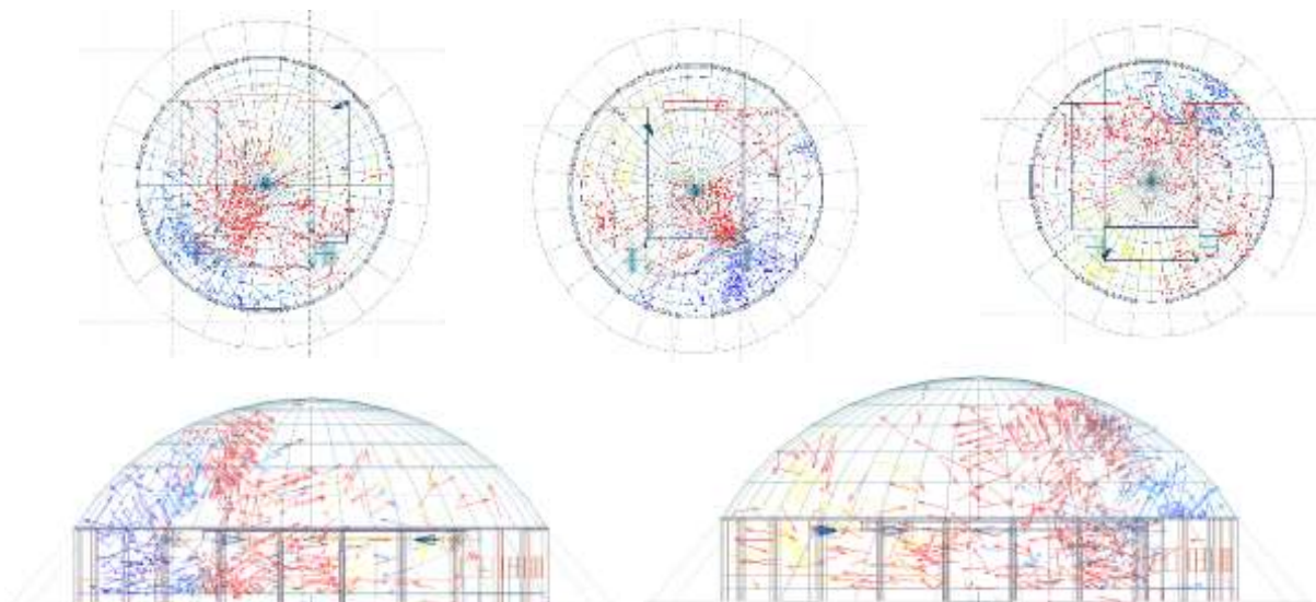
Gambar 6 Simulasi rays and particles speaker (sumber : analisis ecotect)
